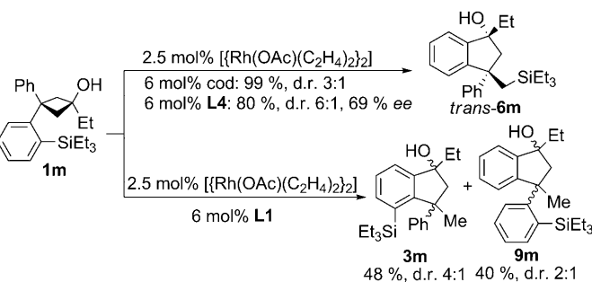
Scheme 4. L4 enables selective C–Si activation of 1m .
